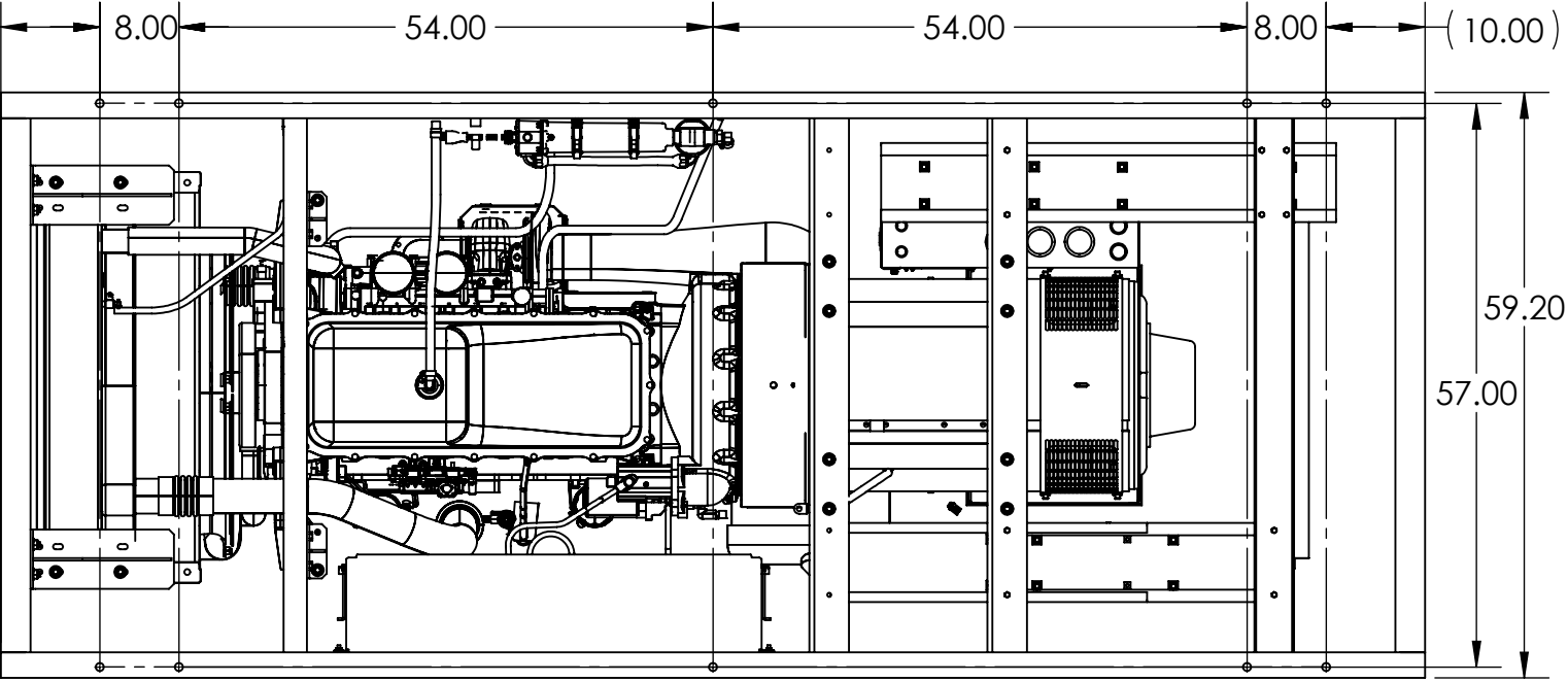
BOTTOM VIEW
