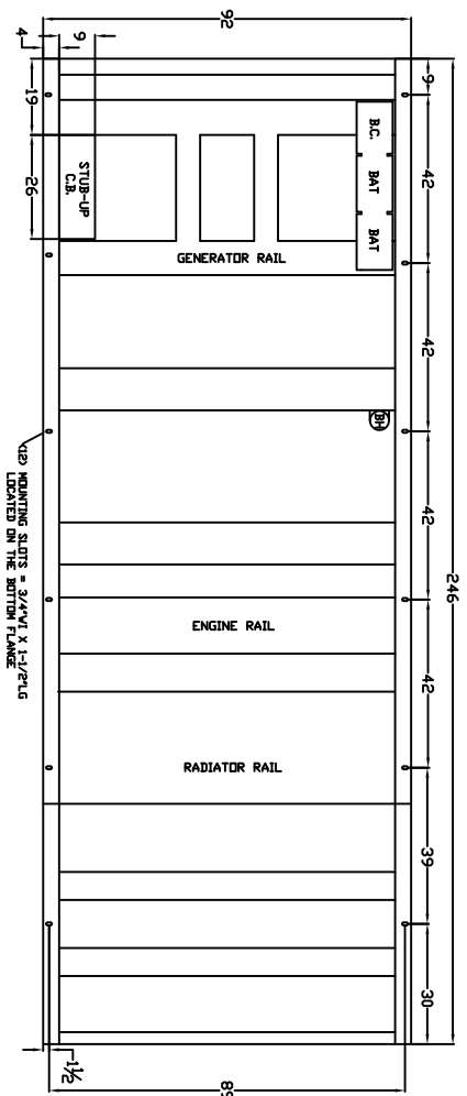
FRAME VIEW
