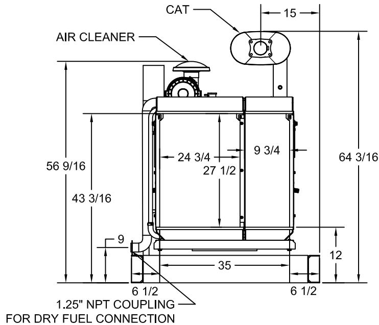
RADIATOR VIEW
